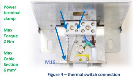
Figure 4 – thermal switch connection
